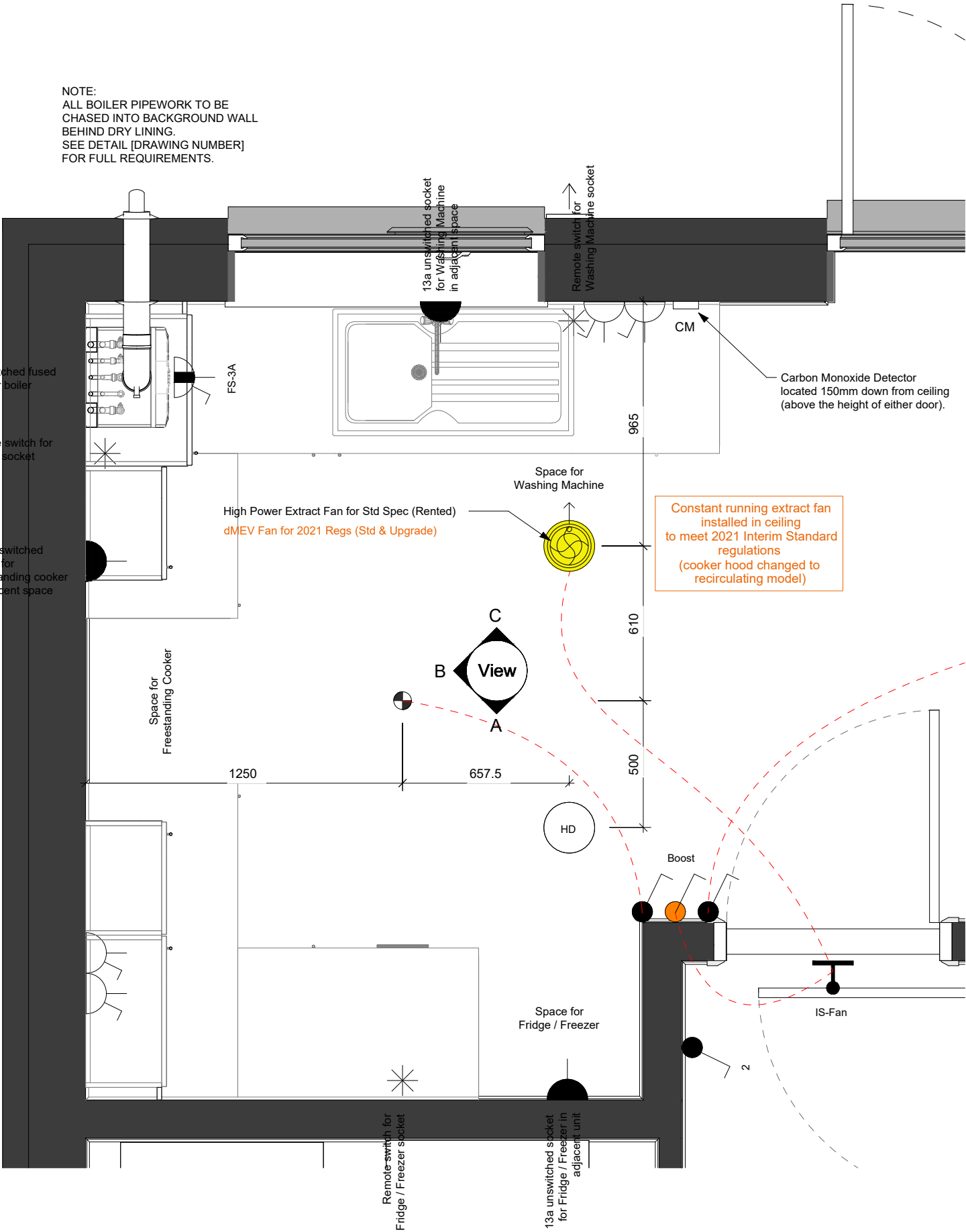
1 Kitchen Layout - Rented Specification 1 : 20
