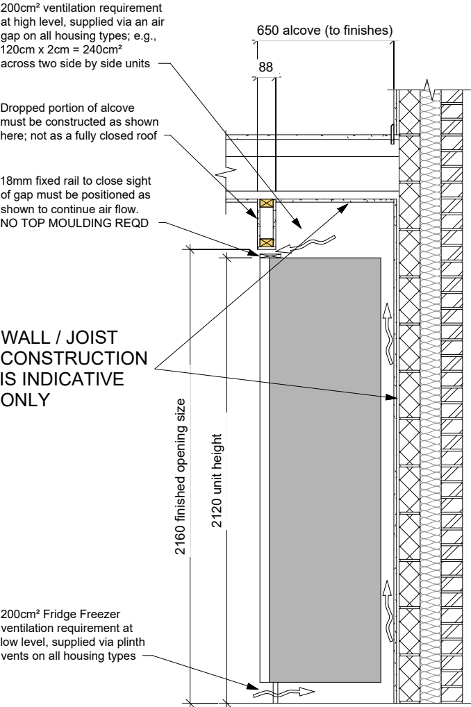
Section through enclosed housing ( 1 : 25)
